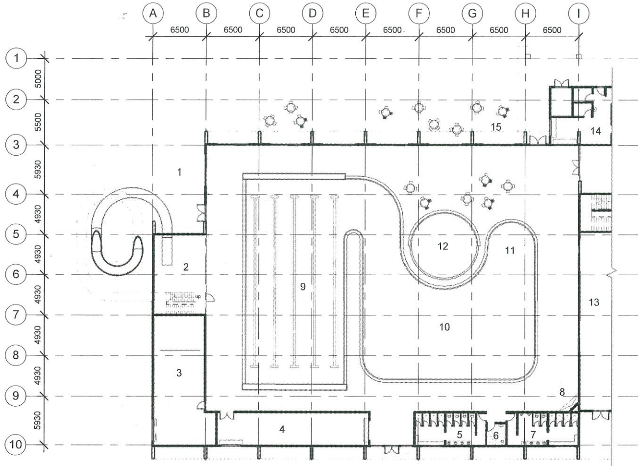
FLOOR PLAN 1
