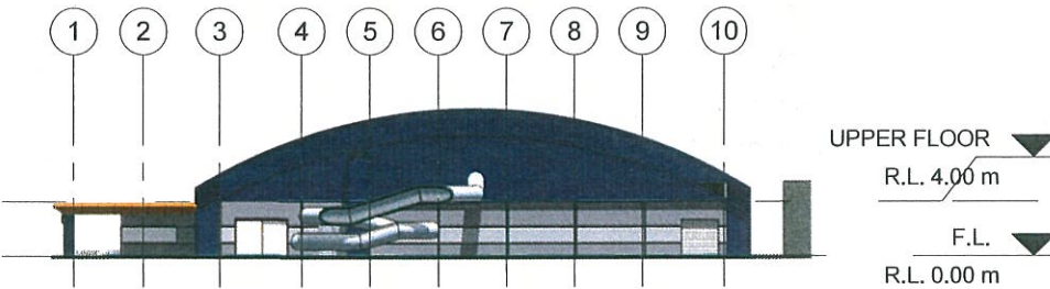
NORTH ELEVATION
