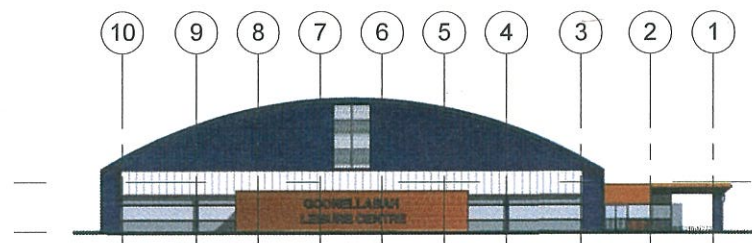
SOUTH ELEVATION
