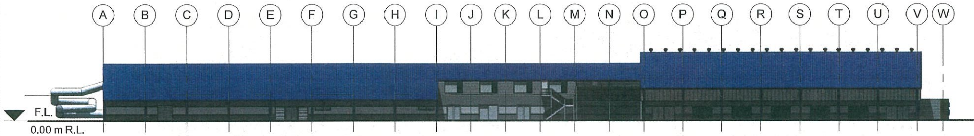
WEST ELEVATION
